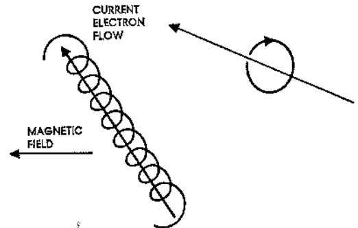
FIGURE XXXIX Magnetic Field.
