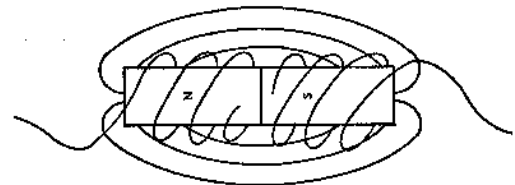
FIGURE XLIII Flow Around Permanent Magnet.
