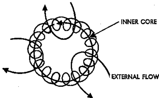
FIGURE XXXI Vortex Ring Circulation.
