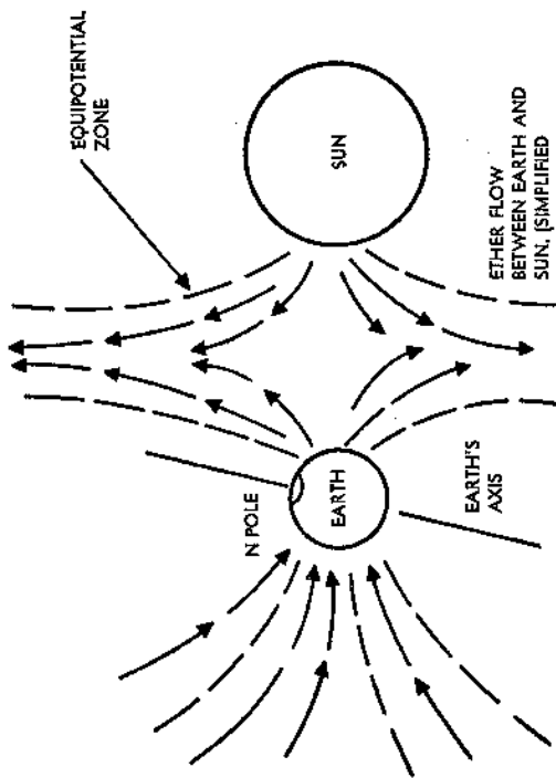
FIGURE XXXVII Gravity Circulation, Earth to Sun.
