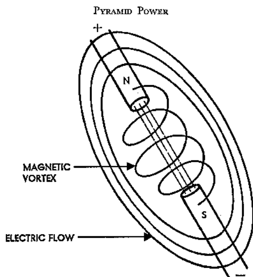
FIGURE XLIV Superimposed Fields.
