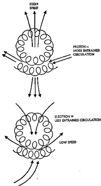
FIGURE XXXIII Ether Circulation in Proton and Electron.
