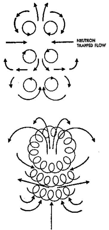
FIGURE XXXIV Circulation in Vortex Neutron
