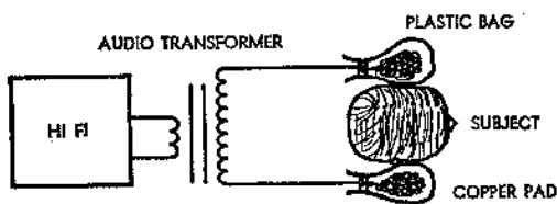
FIGURE V Early experimental Neurophone.
