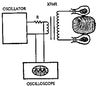
FIGURE VI Measuring resonance.
