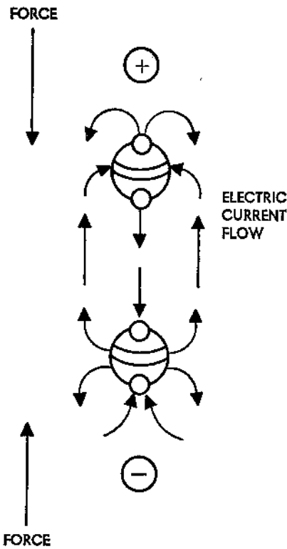
FIGURE XXXVIII Ether Circulation From Electric Charges.
