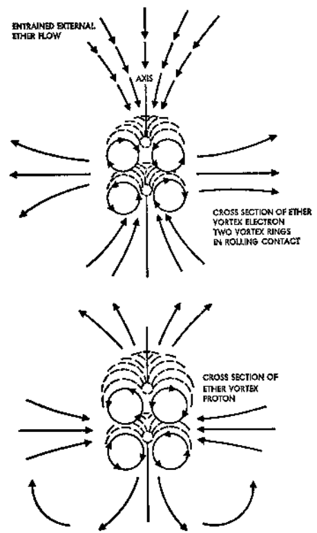
FIGURE XXX Vortex Electron and Proton
