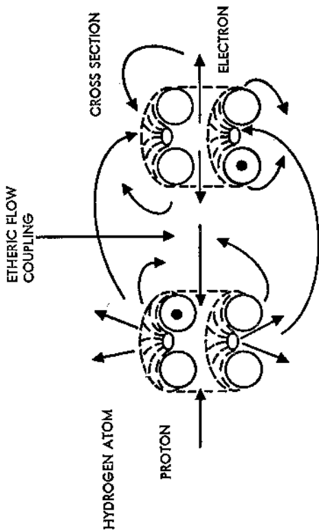
FIGURE XXXV Hydrogen Atom.
