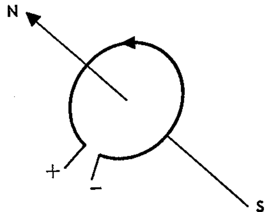
FIGURE XL Magnetic Field Around Loop.
