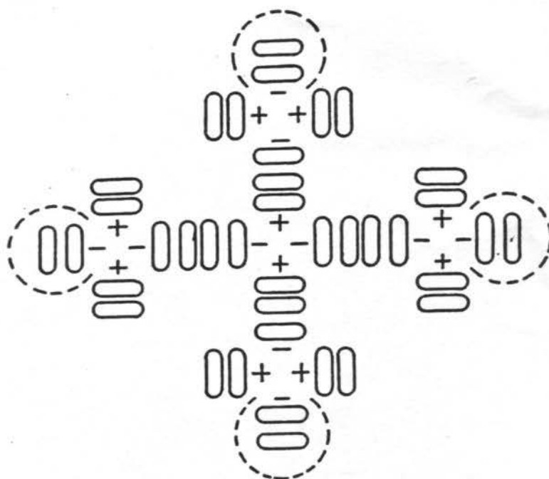
Fig. 5.—The carbon atom. In this and many of the other atoms the number of electrons is not equal to the number of protons, but there is no reason why they should always have to be equal in number to produce electrically neutral structures. Electrification is a surface phenomenon and we have no proof that the usual principles of electrostatics are applicable inside the atoms. In fact, the proton-proton and proton-neutron attractions at close ranges are evidence to the contrary.
