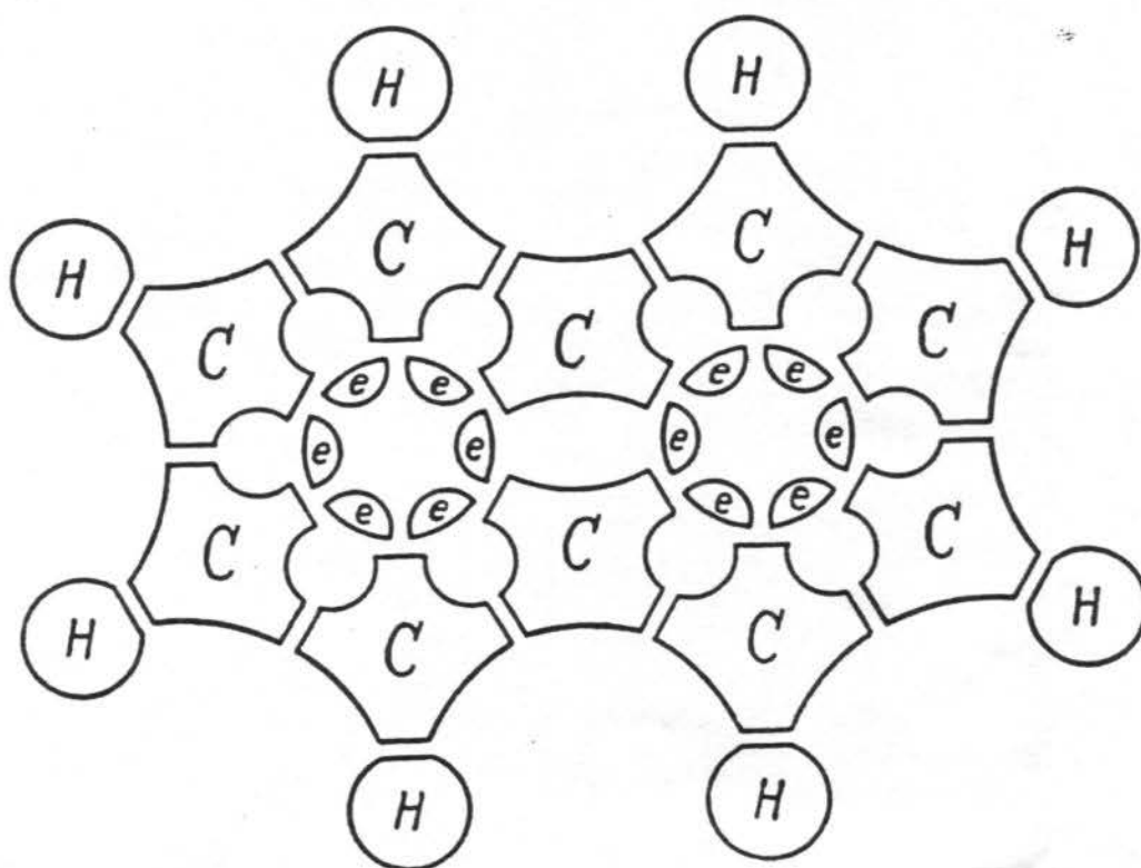
Fig. 8.—The naphthalene molecule with its two inner rings formed of valence electrons e connecting adjacent carbon atoms with one another. The benzene molecule would be an obvious simplification of this structure. The ability of an electron to divide its charge between two adjacent carbon atoms and also the ability of two such electrons to be joined to a single valence bond is demonstrated by the covalent bonds of carbon compounds.
